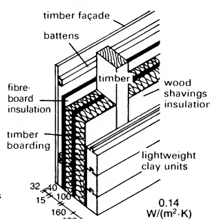
⑪ Timber frame with lightweight clay elements 0.14 W/(m 2 ·K)
